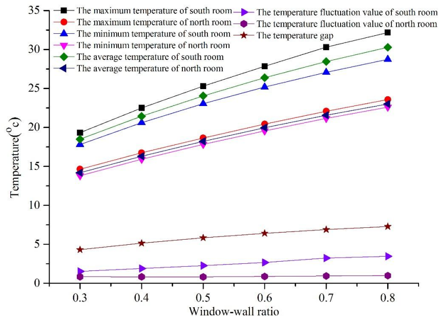
Figure 3. The maximum, minimum, average temperature and temperature difference of south room and north room on the coldest day without heating (°C)
