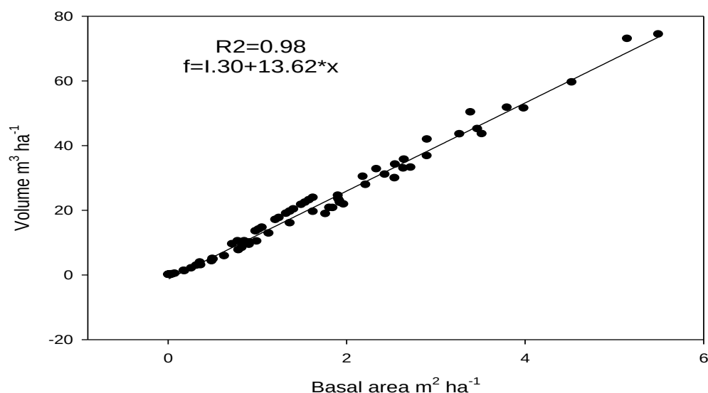
Figure 2. Relationship between volume ( \text{m}^3 \text{ ha}^{-1} ) and basal area \text{m}^2 \text{ ha}^{-1}
