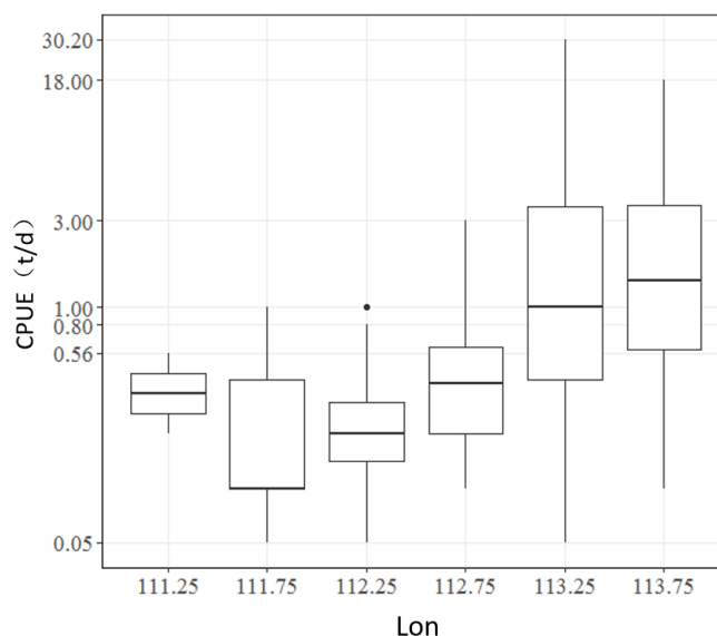
Figure 2. Box plot of longitudinal distribution of D. maruadsi CPUE
