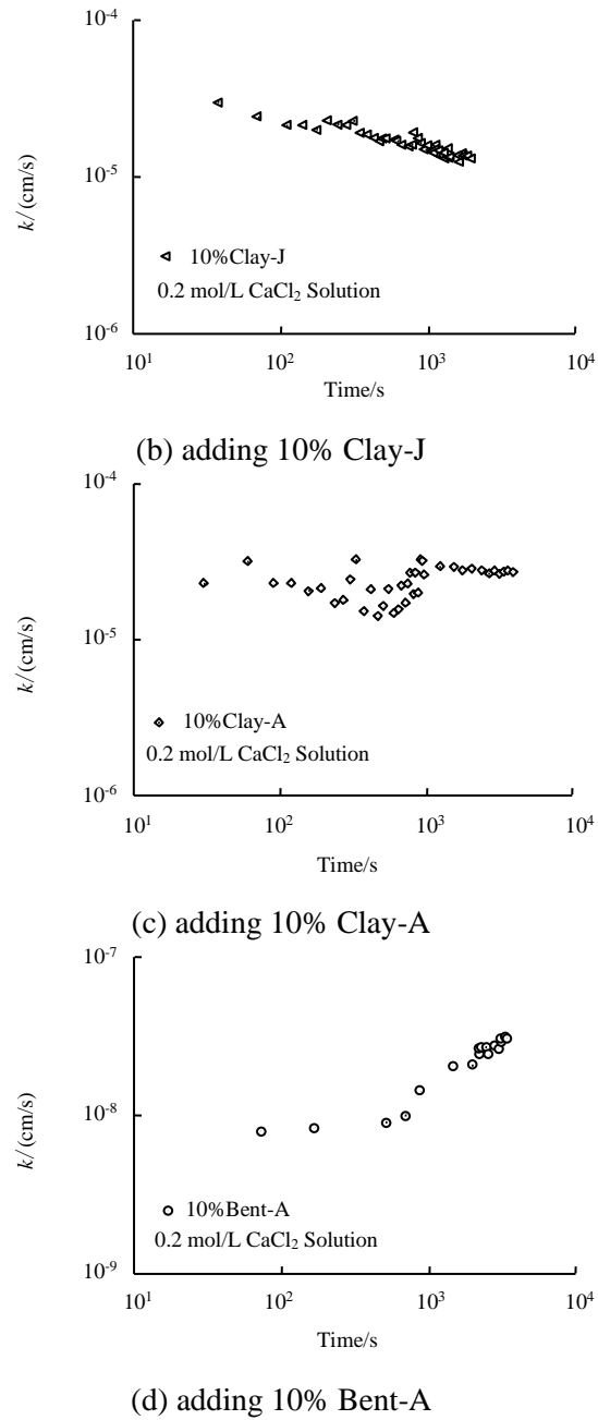
Figure 4. Changes of the hydraulic conductivity of the sand-clay mixtures with time
