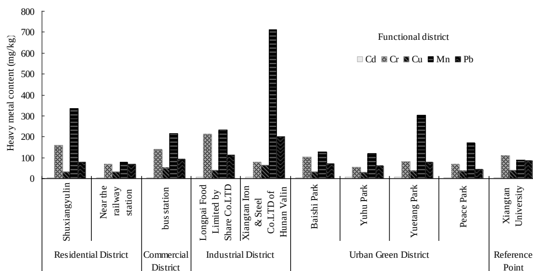
Figure 3. Contents of heavy metals in the barks of Cinnamomum camphora in different functional areas
