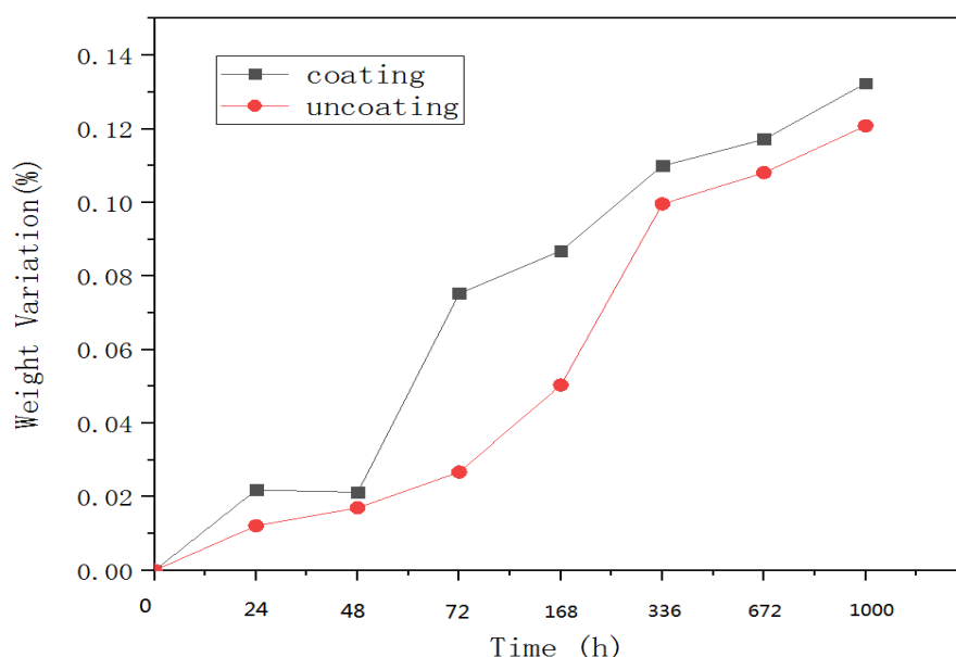
Figure 4. Quality change of composite profile after salt spray test
