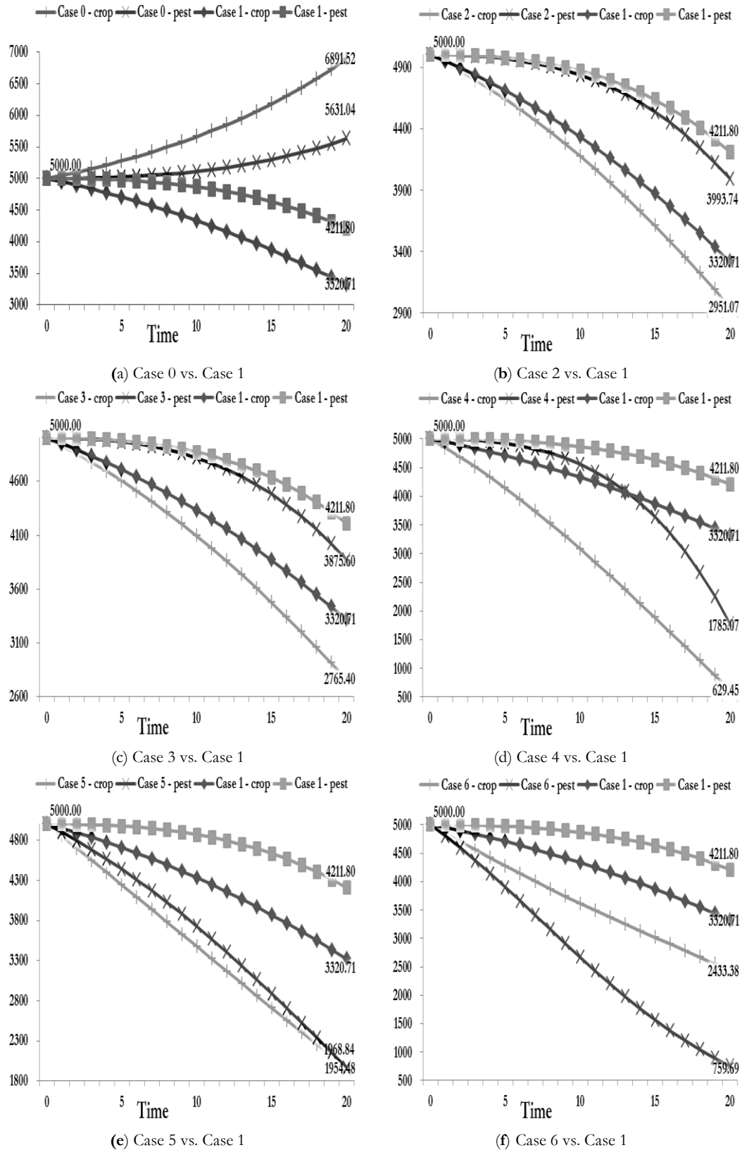
Figure 1. The biodiversity of crop and pest at t = 0 \sim 20 for (a) Case 0 vs. Case 1, (b) Case 2 vs. Case 1, (c) Case 3 vs. Case 1, (d) Case 4 vs. Case 1, (e) Case 5 vs. Case 1, and (f) Case 6 vs. Case 1
