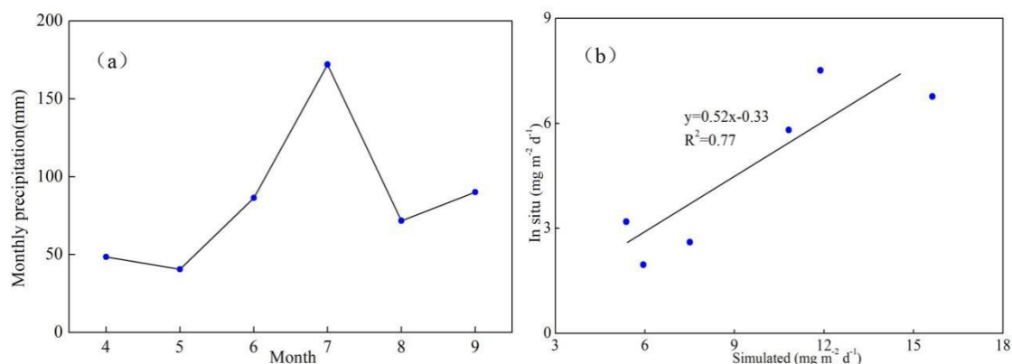
Figure 4. The monthly precipitation (a) and validation results of N emissions (b)
