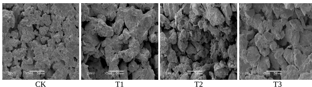
Figure 5. Comparison of soil microstructure under different treatments (500 times). CK is the control treatment applied with inorganic fertilizer, T1, T2 and T3 are treatments applied with biogas slurry of 20, 15 and 10% in volume concentrations, respectively
