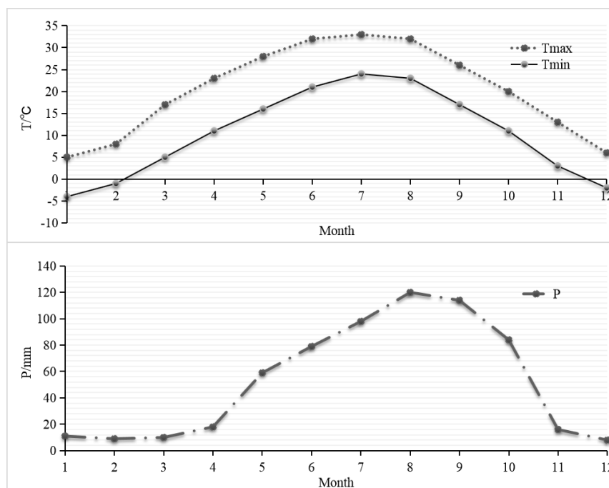
Figure 2. An average temperature and rainfall in the study area from January to December of the year 2016 (Tmax, Tmin and P are represent the an average maximum temperature, anaverage minimum temperature and precipitation of every month)
