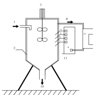
Figure 1. Schematic diagram of the CM AD in CSTR. (1. Feed inlet, 2. Heating layer, 3. Rabblar, 4. pH probe, 5. Oxidation reduction probe, 6. Electrical conductivity probe, 7. Temperature probe, 8. Air outlet, 9. Gas flow indicator, 10. Discharge outlet, 11. Instrument cabinet, 12. Automatic monitoring instrument for methane analysis)
