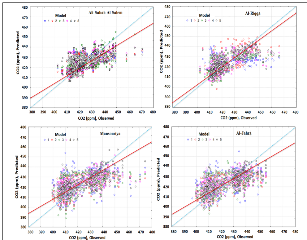
Figure 5. Comparisons between the observed and predicted daily \text{CO}_2 emissions at all sites in 2016. The dashed line is the 1:1 line, and the solid line is the best-fit line
