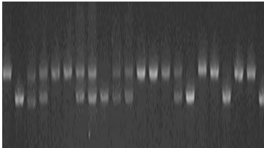
Figure 2. Amplification results
