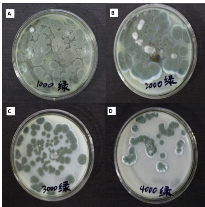
Figure 1. The growth status of Penicillium sp. Pb-G in medium with different concentrations of \text{Pb}^{2+} . A, 1000 mg/L; B, 2000 mg/L; C, 3000 mg/L; D, 4000 mg/L
