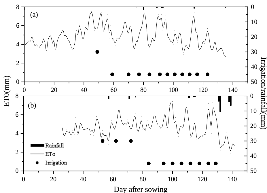
Figure 4. Daily reference crop evapotranspiration ( ET_0 ), rainfall, and irrigation at the experimental site during the 2014 and 2015 seasons
