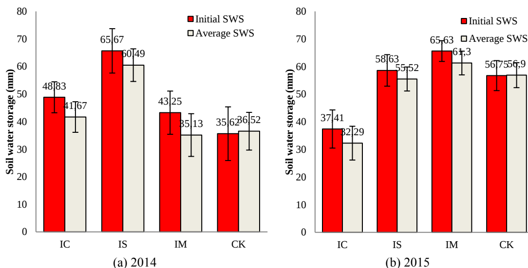
Figure 5. The initial and average SWS at 40 cm depth for the different treatments in 2014 and 2015.
