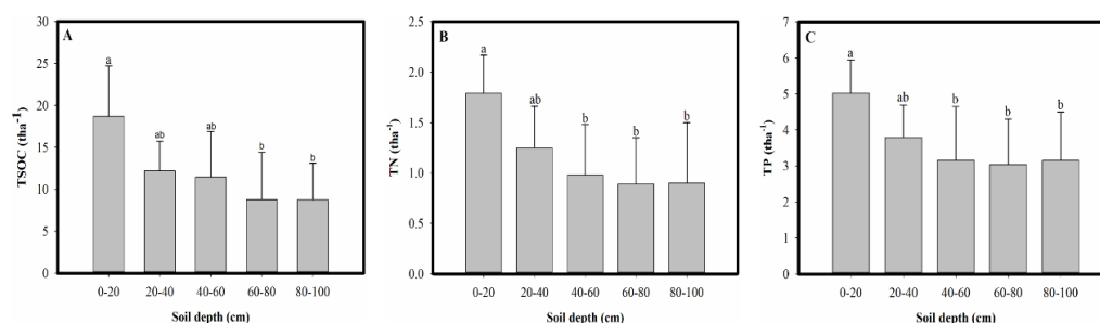
Figure 4. Mean values of total soil organic carbon ( t\ ha^{-1} ) (a), total nitrogen ( t\ ha^{-1} ) (b) and total phosphorous ( t\ ha^{-1} ) (c) along the depth increment. TSOC, TN, and TP indicate the total soil organic carbon, total nitrogen, and total phosphorous. Values are mean \pm standard deviation, different alphabets on each error bar denote the significant differences ( p < 0.01 , n=7 ) at a given soil depth
