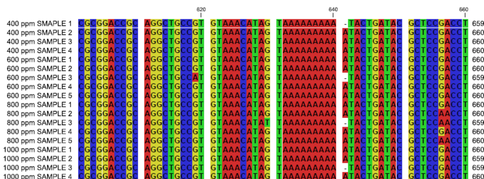
Figure 2. Sequence alignment of ITS region of M. persicae individuals grown at ambiante and elevated CO 2 levels. Mutational sites of ITS region of M. persicae grown at 800 ppm CO 2 level are boxed
