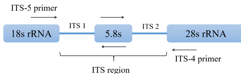
Figure 1. Diagram of nuclear ribosomal RNA (nrRNA) gene containing ITS1, 5.8S, and ITS2 regions with primer binding sites
