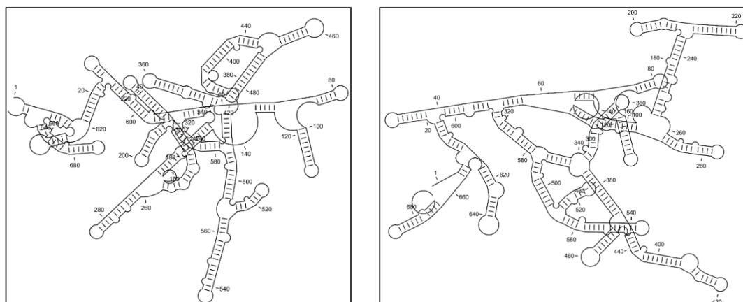
Figure 4. The most stable secondary structure based on 730 bp of consensus ITS sequence of green peach aphids grown at ambient CO 2 (A) and elevated (600, 800 (B) and 1000 ppm) CO 2 levels
