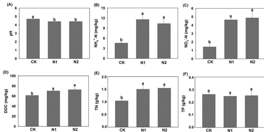
Figure 1. Effects of N addition on soil properties. Values are mean ± standard errors ( n=3 ). \text{NH}_4^+\text{-N} : ammonium-N; \text{NO}_3^-\text{-N} : nitrate-N; DOC: dissolved organic carbon; TN: total nitrogen; TP: total phosphorus. Different letters indicate significant differences among N fertilizer treatments ( P < 0.05 )
