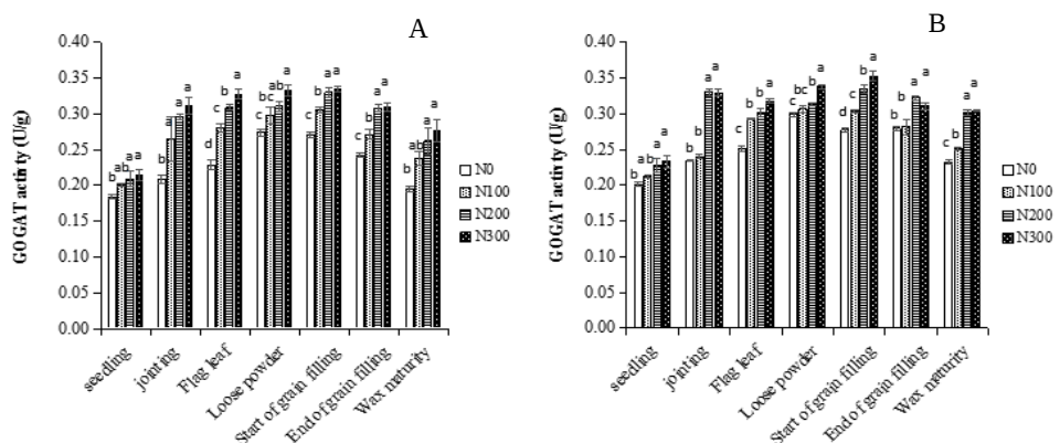
Figure 4. Effect of nitrogen on GOGAT activity of sorghum leaf (A) 2016, (B) 2017. Different letters indicate different means, according to LSD test ( p < 0.05 )
