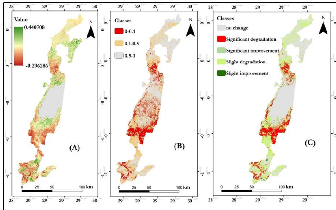
Figure 5. a) Annual change trends in NDVI, b) Significance (P-Value) of the change trends in NDVI, c) The overall trends classified in into five types: significant improvement, slight improvement, stable or no vegetated, slight degradation and significant degradation
