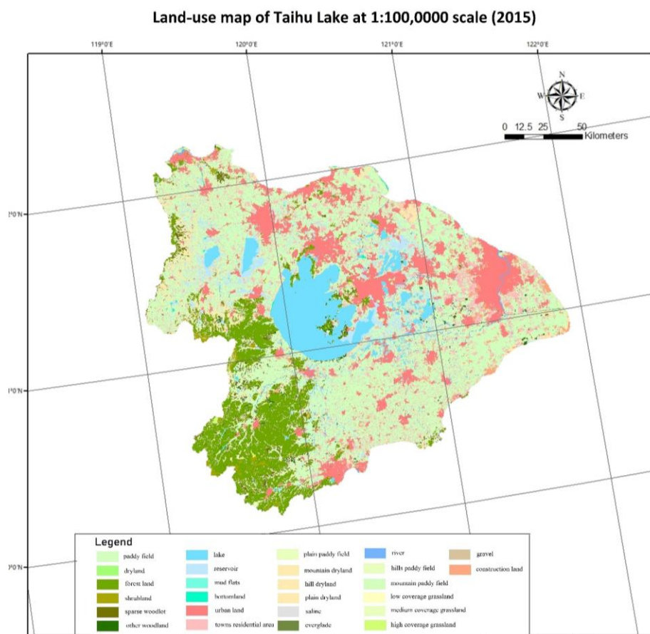
Figure 2. Land-use map of Taihu Lake basin at 1:100,000 scale (2015)
