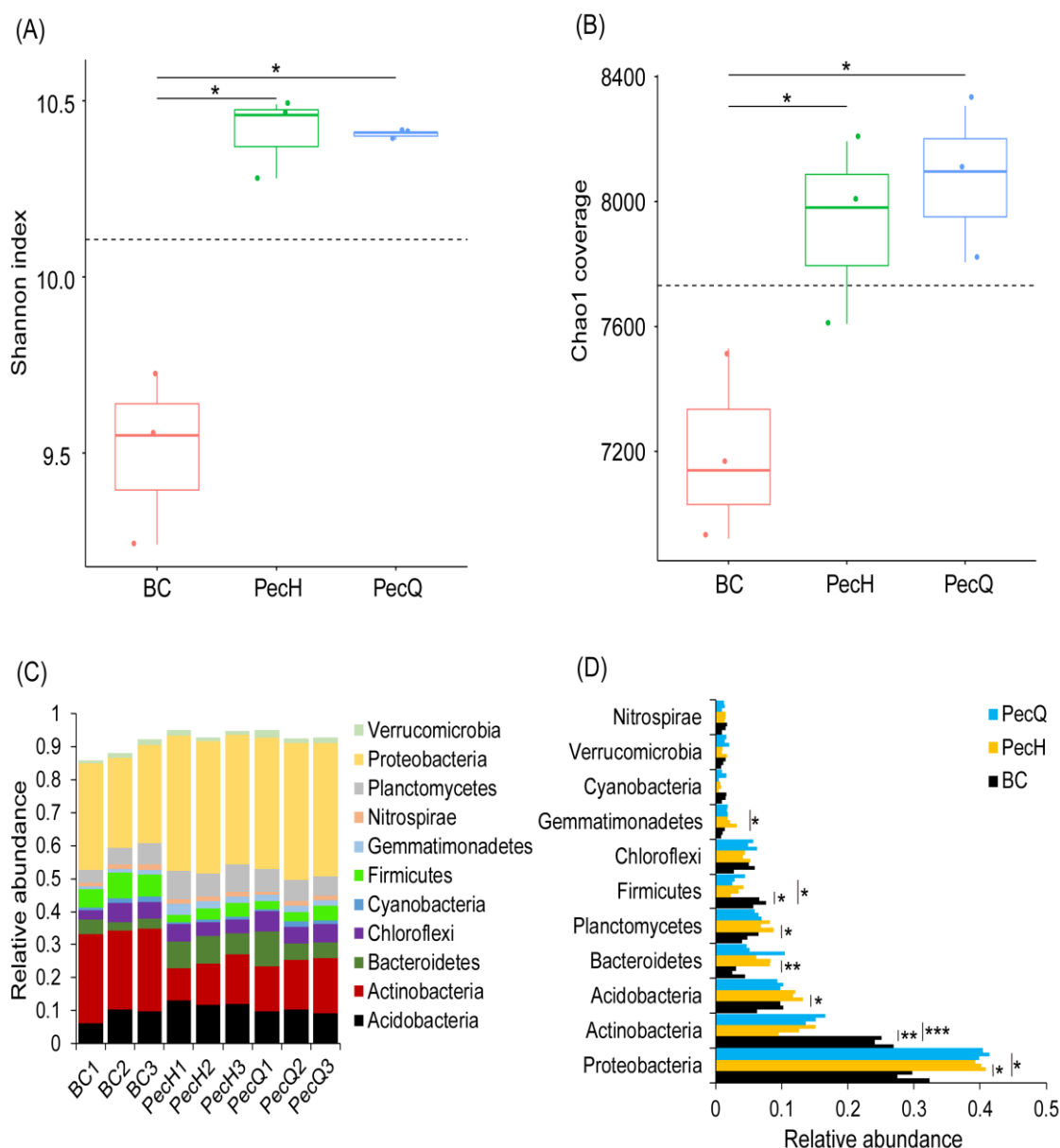
Figure 6. The Shannon index (A), Chao1 coverage (B), dominant phylum compositions (C), and dominant phylum differences in the rhizosphere microbiome among different treatments (D). BC, blank control; PecH, the samples before infection with Pectobacterium sp. MB001; PecQ, the samples after infection with Pectobacterium sp. MB001. * p < 0.05 , ** p < 0.01 , *** p < 0.001
