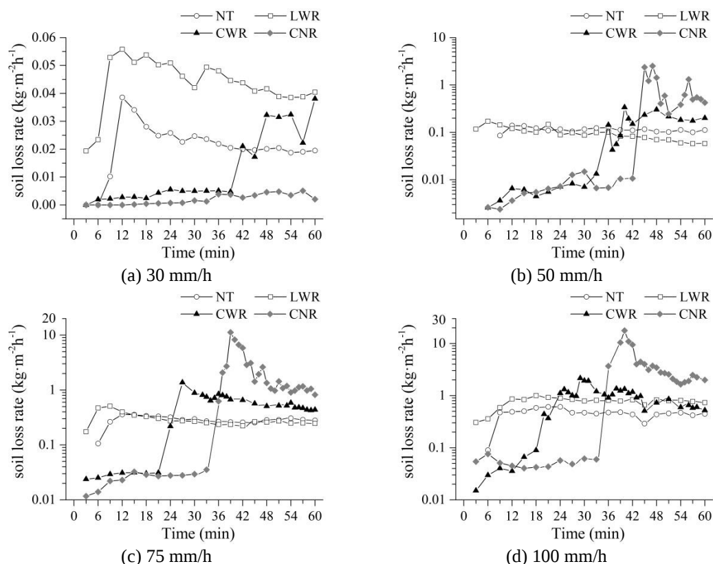
Figure 8. Changes in soil loss rate under various tillage practices under different rainfall intensities. Note: the average soil loss rate is the average value of soil loss rates under 3^\circ and 5^\circ under this tillage practice
