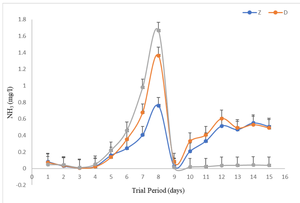
Figure 3. \text{NH}_3 exchange during the experimental period (15 days)
