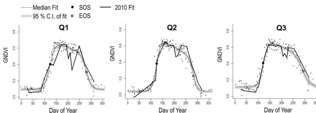
Figure 5. The temporal dynamics of GNDVI on the sites dominated by Quercus robur L. in the Ufa city and outside it. Q1 – outside the city, Q2 – in the city on a flat area, Q3 – in the city on a steep southern slope; Median Fit – average plot of 2008-2017; 95% C.I. of fit – 95% credible interval of median fit; SOS – start of season; EOS – end of season; 2010 Fit – plot of 2010
