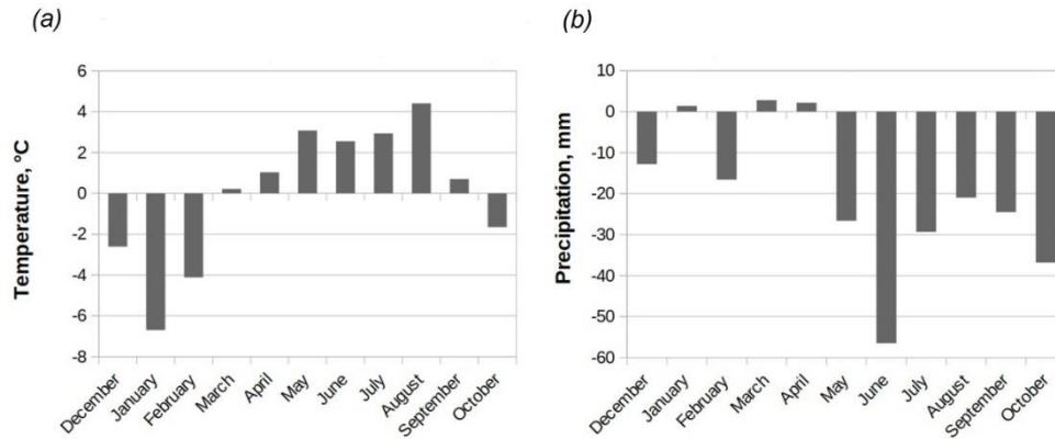
Figure 2. Deviation from the average values: a) monthly average temperature (from December of the previous year to October of the year under review) in the dry year 2010 from the average values for the last 70 years (1950-2019); b) average monthly precipitation (from December of the previous year to October of the year under review) in the dry year 2010 from the average values for the last 70 years (1950-2019)
