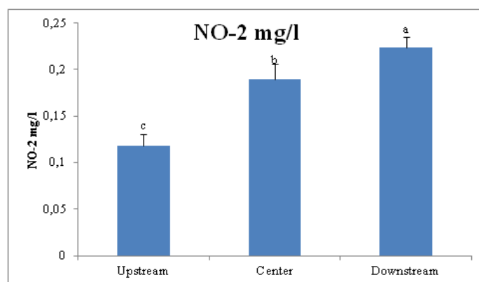
Figure 7. Spatial variation of \text{NO}_2^-
