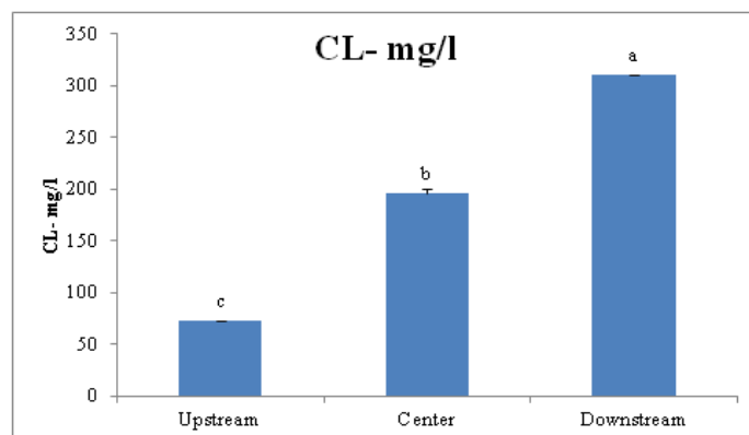
Figure 8. Spatial variation of Cl -
