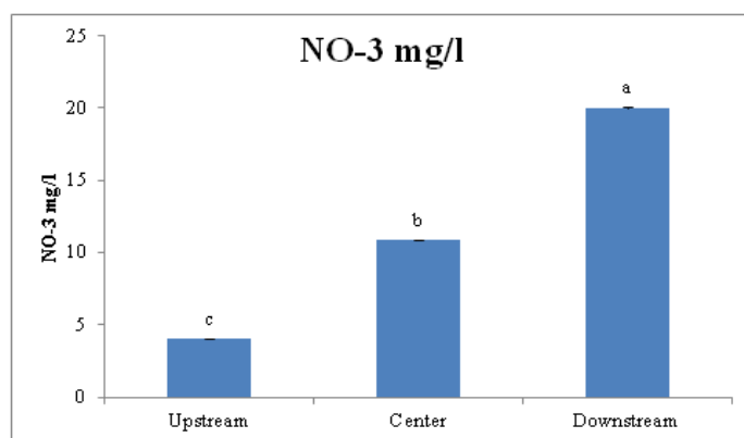
Figure 6. Spatial variation of \text{NO}_3^-
