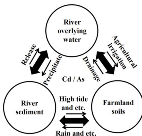
Figure 5. Potential migration routes of Cd and As in the vegetable soil along the River
