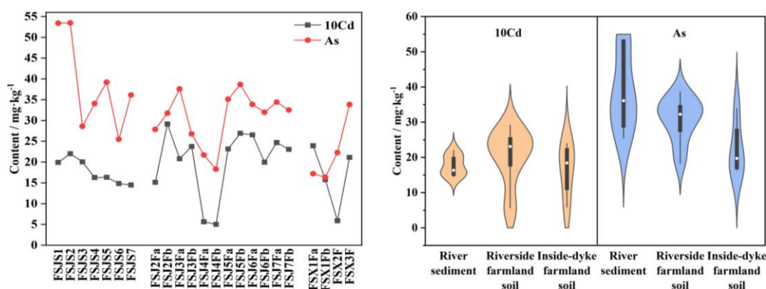
Figure 2. Content distribution of Cd and As in the river sediment and the farmland soil
