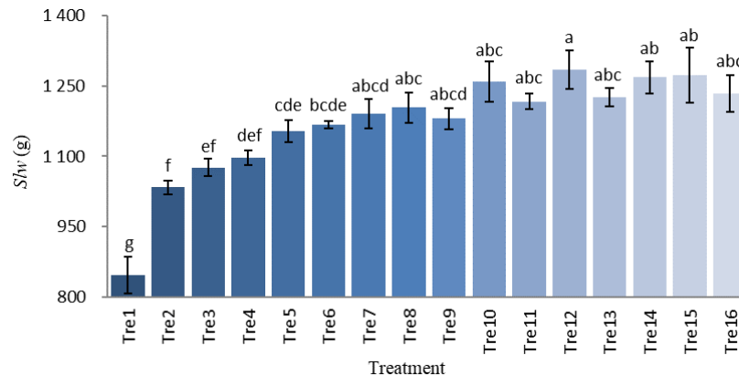
Figure 2. branch and leaf oven-dried weight of Zanthoxylum armatum ‘Hanyuan Putao Qingjiao’. Slw -Shoots & leaf weight
