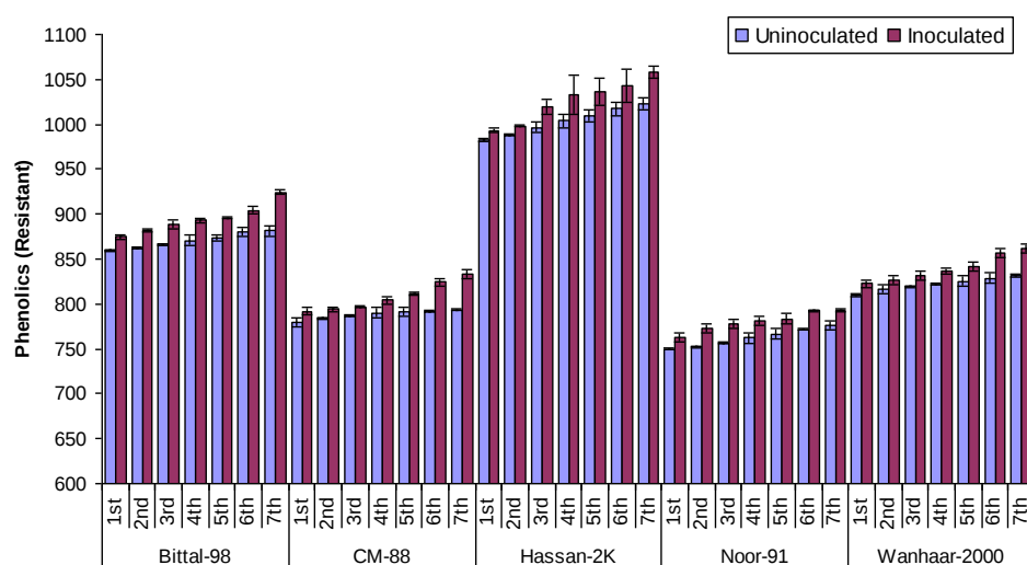
Figure 5. Effect of M. incognita on total phenolic contents in five resistant chickpea genotypes i.e., Bittal-98, CM-88, Hassan-2K, Noor-91 and Wanhhaar-2000
