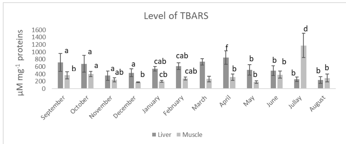
Figure 9. TBARS level ( \mu\text{M mg}^{-1} proteins) in muscle and liver of Boops boops fish, from Oran Bay. The different letters (a, b, c, e, f, d, k) designate significant differences between Level of TBARS in organ and month (Fischer's LSD test ( P < 0.05 ))
