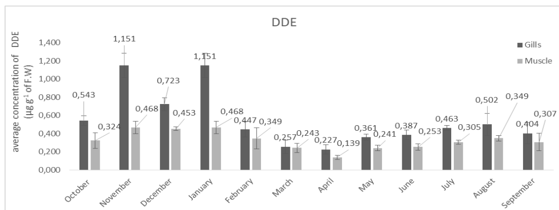
Figure 7. Average levels of DDE, ( n = 5 , mean \pm SD) evaluated in muscle and gills ( \mu\text{g g}^{-1} of F.W) of bogue from Oran Bay
