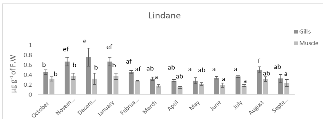
Figure3. Monthly variations of Lindane levels evaluated in muscle and gills ( \mu\text{g g}^{-1} of F.W) of bogue from Oran Bay ( n = 5 , mean \pm SD). The different letters (a, b, e, f) designate significant differences between OCPs in organ and month (Fischer's LSD test ( P < 0.05 ))
