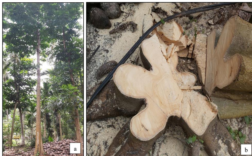
Figure 1. a) Pterygota alata tree grown in farm condition b) collection of Pterygota alata wood samples from the farm
