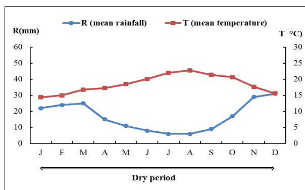
Figure 3. Diagram of Gaussen and Bagnouls applied for Sidi Ifni region ( https://fr.climate-data.org )
