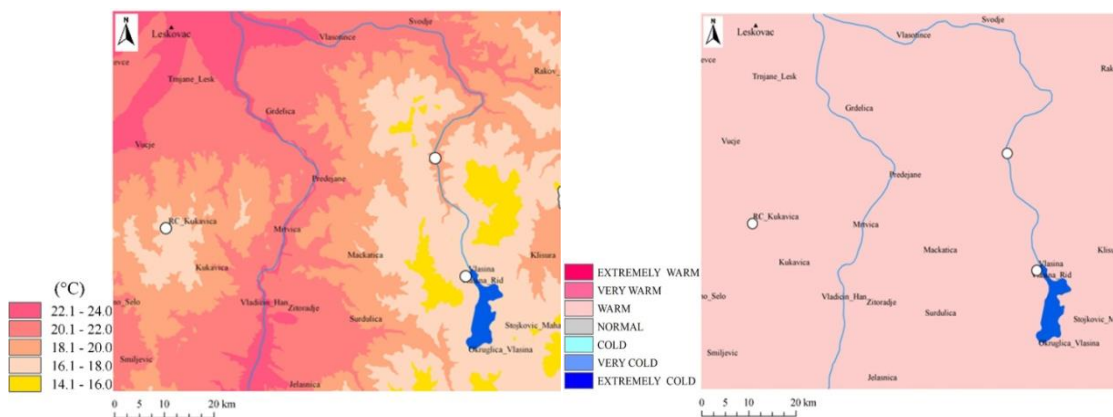
Figure 5. The spatial distribution of mean daily air temperatures for August 18 th (left) and based on the percentile method (right) in relation to the referential period 1991-202
