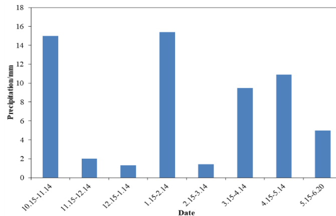
Figure 1. Precipitation amount
