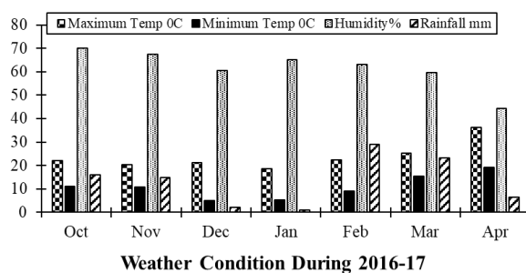
Figure 1. Weather details of experimental site
