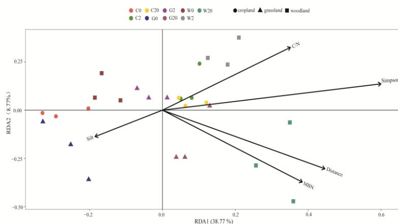
Figure 9. RDA (redundancy analysis) using soil microbial activity, soil texture, soil stoichiometric ratio and vegetation biodiversity indices to explain variation of soil properties in reservoir buffer strips with three land use types and distance from watercourse. The variables presented were determined by a combination of forward selection and backward selection. Points are colored based on different site with symbols distinguishing land use types (circle = cropland, triangle = grassland, diamond = woodland). Abbreviation for selected variables: Distance (distance form watercourse); Silt (silt content); MBN (microbial biomass nitrogen); C/N (carbon nitrogen ratio); Simpson (Simpson index)
