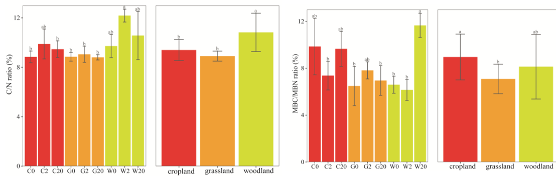
Figure 5. Soil stoichiometric ratio{Soil carbon nitrogen ratio (C/N), Soil microbial carbon nitrogen ratio (MBC/MBN)} of reservoir buffer strips with different land use types. Left: Soil stoichiometric ratio between different sites. Different lowercase letters indicate levels of statistical significance of soil stoichiometric ratio between different sites ( p < 0.05 ). Right: Soil stoichiometric ratio between different land use types. Different lowercase letters indicate levels of statistical significance of soil stoichiometric ratio between different land use types ( p < 0.05 ). The vertical bars represent means, and the error bars represent standard errors
