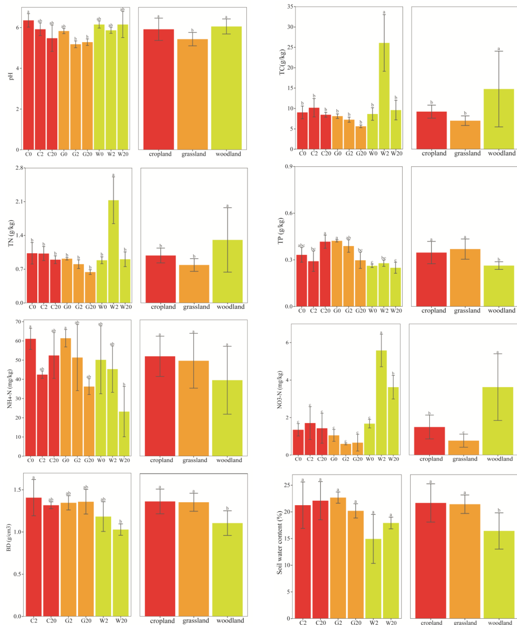
Figure 2. Soil properties {pH, total carbon (TC), total nitrogen (TN), and total phosphorus (TP), ammonium nitrogen ( \text{NH}_4\text{-N} ), and nitrate nitrogen ( \text{NO}_3\text{-N} ), bulk density (BD), soil water content (SWC)} of reservoir buffer strips with three land use types. Left: Soil properties between different sites. Different lowercase letters indicate levels of statistical significance of soil properties between different sites ( p < 0.05 ). Right: Soil properties between three land use types. Different lowercase letters indicate levels of statistical significance of soil properties between different land use types ( p < 0.05 ). The vertical bars represent means, and the error bars represent standard errors
