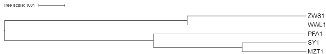
Figure 5. UPGMA clustering results between groups
