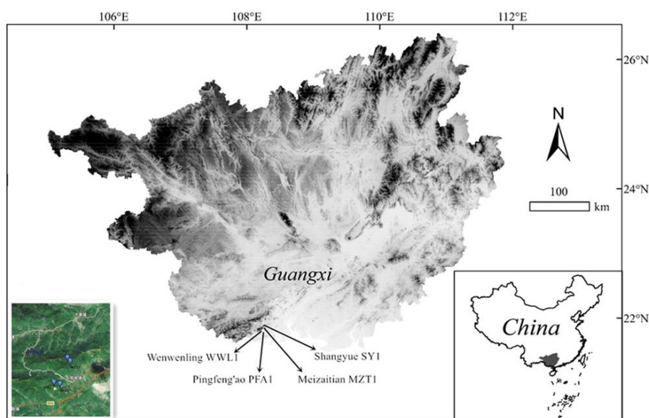
Figure 1. Wild distribution and collection sites of C. shiwandashanica in Shiwandashan Mountains. The map can be downloaded from the Geospatial Data Cloud ( https://www.gscloud.cn )
