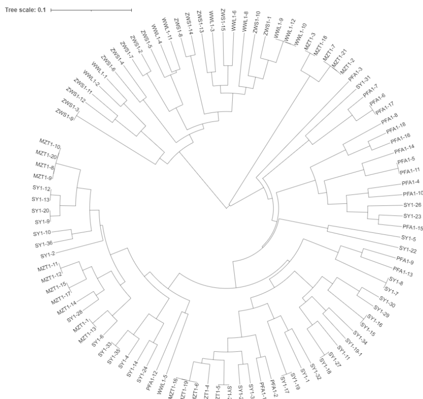
Figure 6. UPGMA clustering results between individuals
