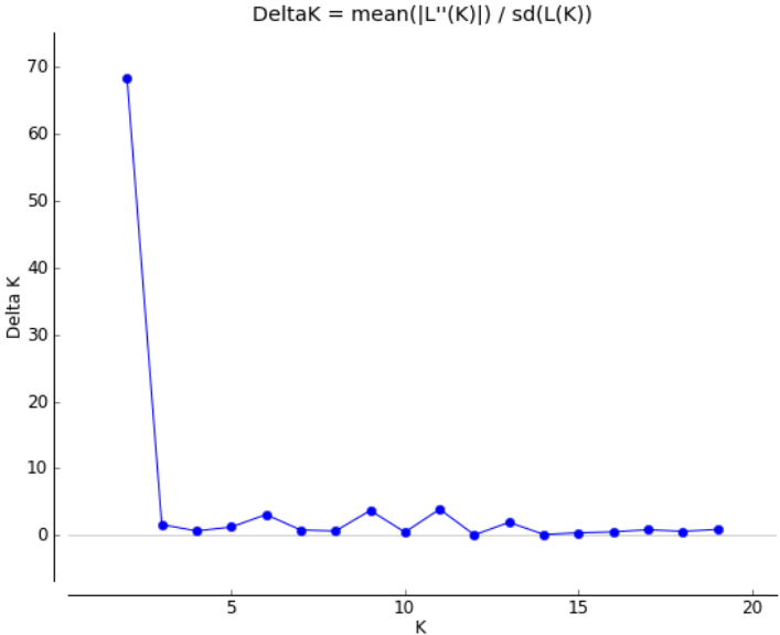
Figure 3. K value change graph drawn by \Delta K method of structure analysis
