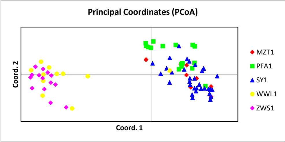
Figure 2. Principal coordinate analysis of samples
