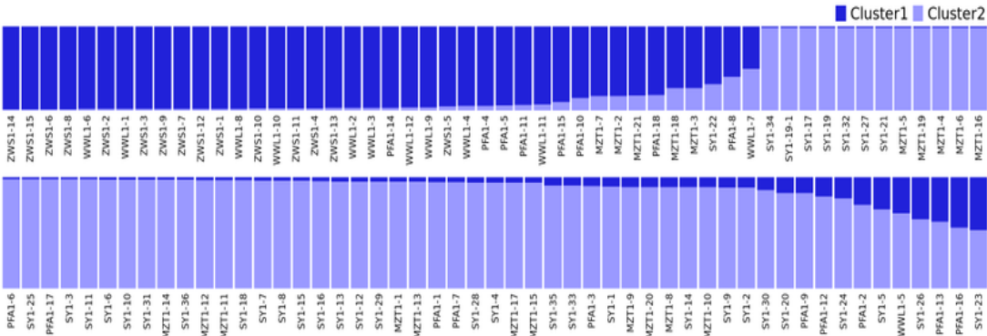
Figure 4. structure results of samples at K=2
