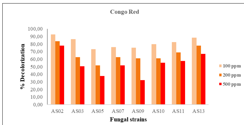
Figure 4. PVM percentage decolorization of CR dye by microfungal strains from Ain Skhouna wetland
