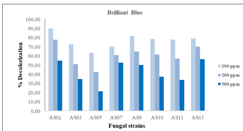
Figure 5. PVM percentage decolorization of BB dye by microfungal strains from Ain Skhouna wetland
