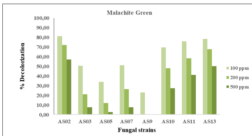
Figure 6. PVM percentage decolorization of MG dye by microfungal strains from Ain Skhouna wetland
