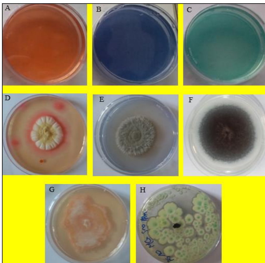
Figure 9. Dyes decolorization mechanisms for microfungi strains of Ain Skhouna. A, B and C: negative controls 500 ppm of CR, BB and MG. D: adsorption of CR to the mycelium of A. iranicus strain AS03. E: biodegradation of BB by H. carbonneanum strain AS09. F: biodegradation of MG by Aspergillus sp. strain AS02. G: absorption of CR by F. acuminatum strain AS07. H: accumulation of MG by Penicillium sp. AS10 strain
