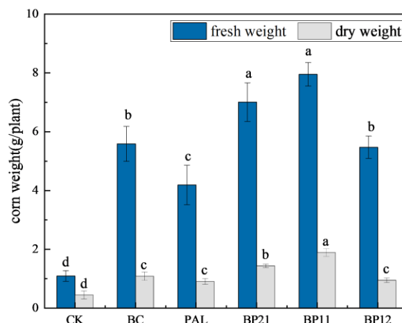
Figure 11. The corn fresh and dry weight harvested from the soil treated with various stabilizers. Data were means \pm SD ( n = 3 ). Column with the different letter has significant differences among all treatments at according to the Duncan's test ( P < 0.05 )
