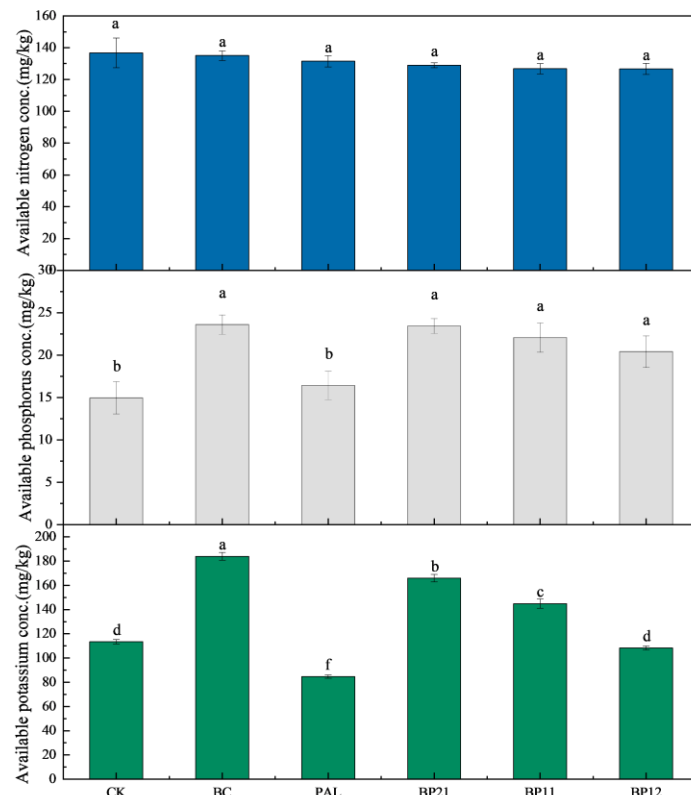
Figure 7. Effect of stabilizers on available nutrients contents of soil. Data were means \pm SD ( n = 3 ). Column with the different letter has significant differences among all treatments at according to the Duncan's test ( P < 0.05 )
