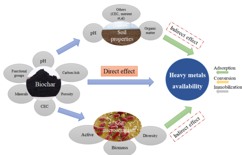
Figure 1. The effects of biochar on available heavy metals in the contaminated soil
