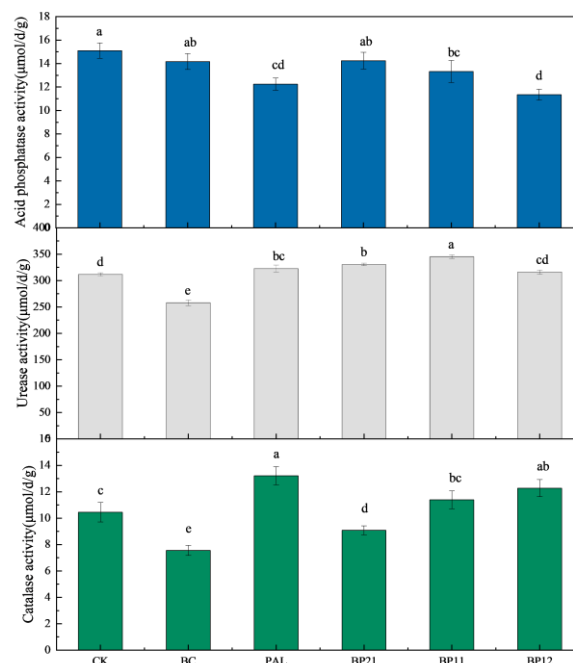
Figure 6. Effect of stabilizers on enzymatic activity of soil. Data were means \pm SD ( n = 3 ). Column with the different letter has significant differences among all treatments at according to the Duncan's test ( P < 0.05 )
