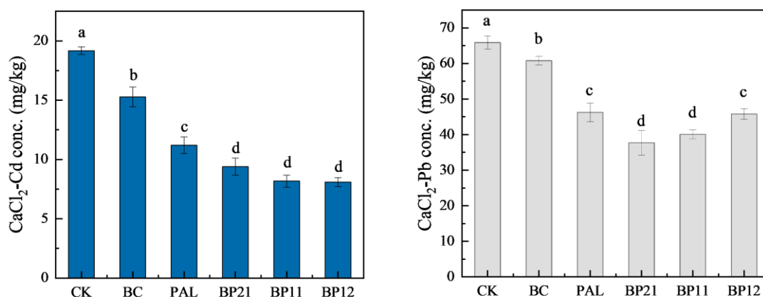
Figure 9. The \text{CaCl}_2 -extractable Cd and Pb in the soil treated with various stabilizers. Data were means \pm SD ( n = 3 ). Column with the different letter has significant differences among all treatments at according to the Duncan's test ( P < 0.05 )
