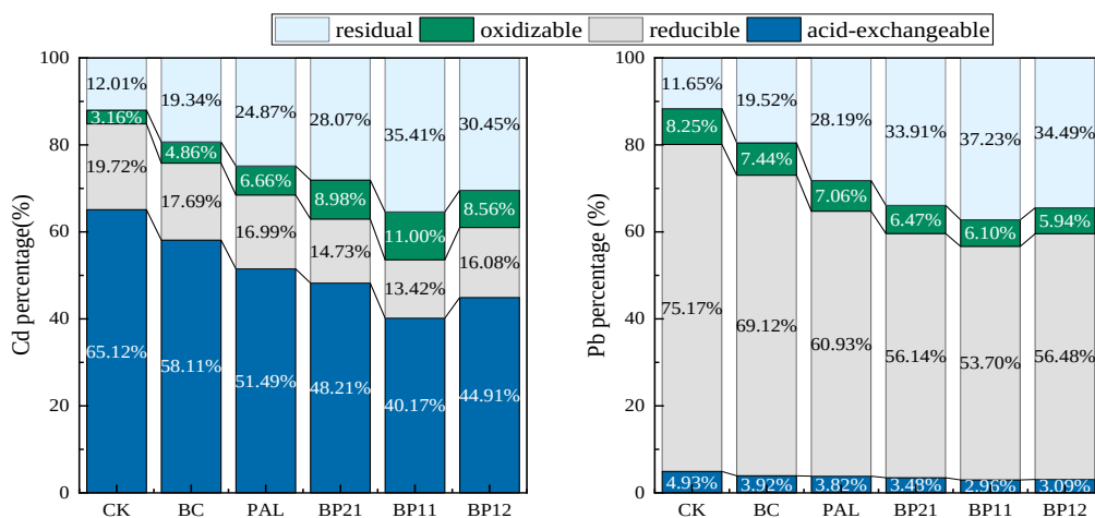
Figure 10. The fractions of different Cd and Pb speciation in soil treated with various stabilizers
