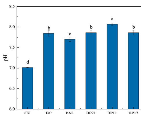
Figure 5. Effect of stabilizers on soil pH. Data were means \pm SD ( n = 3 ). Column with the different letter has significant differences among all treatments at according to the Duncan's test ( P < 0.05 )
