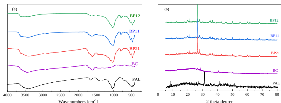
Figure 3. (a) FT-IR spectra and (b) XRD patterns of BC, PAL, BP21, BP11 and BP12
