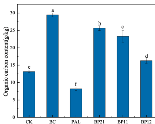
Figure 8. Effect of stabilizers on organic carbon content of soil. Data were means \pm SD ( n = 3 ). Column with the different letter has significant differences among all treatments at according to the Duncan's test ( P < 0.05 )
