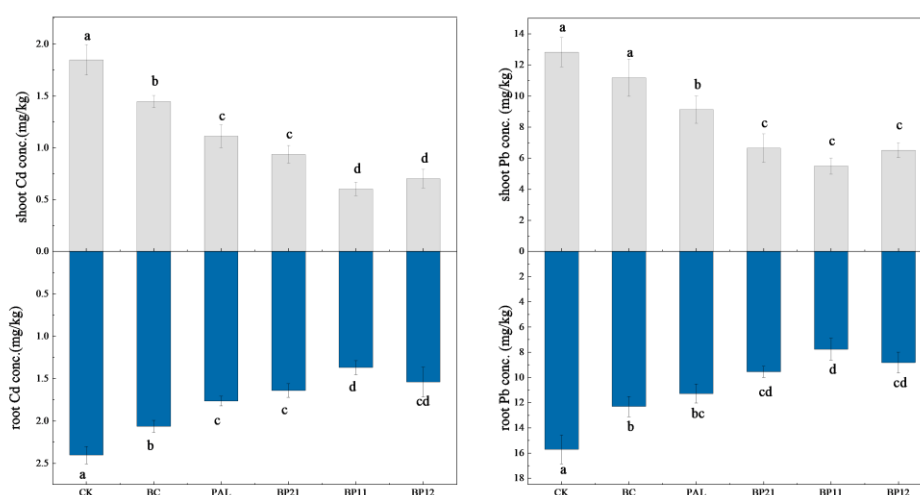
Figure 12. Concentration of Cd and Pb in corn shoots and roots part harvested from the soil treated with various stabilizers. Data were means \pm SD ( n = 3 ). Column with the different letter has significant differences among all treatments at according to the Duncan's test ( P < 0.05 )
