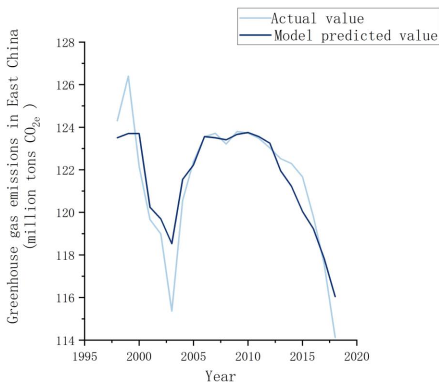
Figure 6. Model validation in Eastern China from 1998 to 2018
