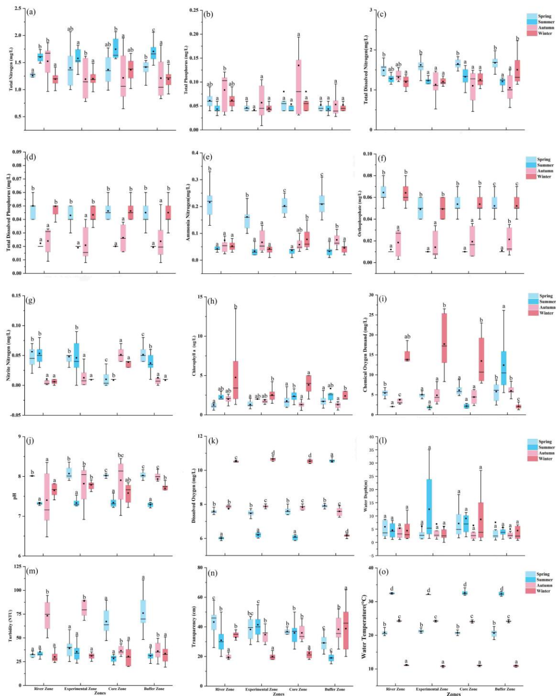
Figure 2. Seasonal patterns of (a) total nitrogen, (b) total phosphorus, (c) total dissolved nitrogen, (d) total dissolved phosphorus, (e) ammonia nitrogen, (f) orthophosphate, (g) nitrite nitrogen, (h) chlorophyll a , (i) chemical oxygen demand, (j) pH, (k) dissolved oxygen, (l) water depth, (m) turbidity, (n) transparency, and (o) water temperature in the regions. Note: bars with different lowercase letters indicate significant differences among seasons
