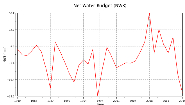
Figure 1. The change of the global average Net Water Budget between 1980 and 2015
