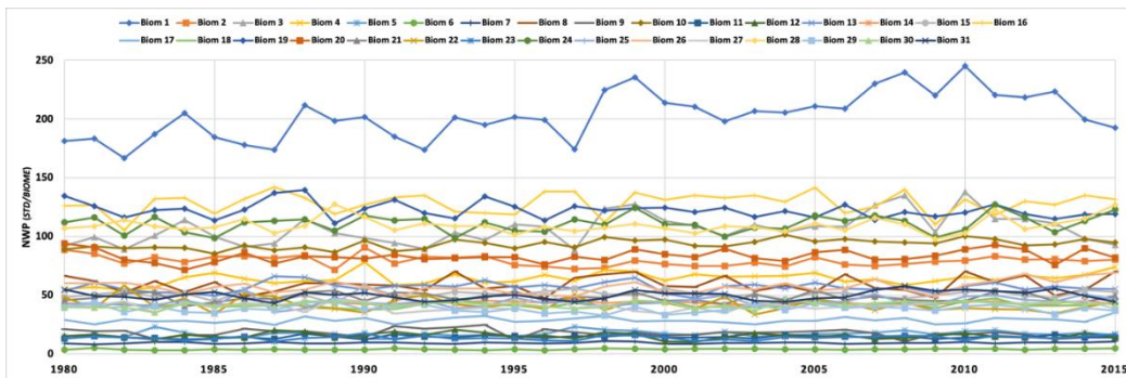
Figure 8. Standard deviation of Net Water Budget per biome group (NWP) from 1980 to 2015
