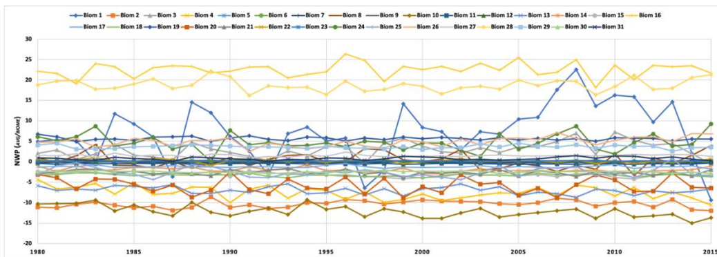
Figure 7. Global average of Net Water Budget per biome (NWP) group from 1980 to 2015
