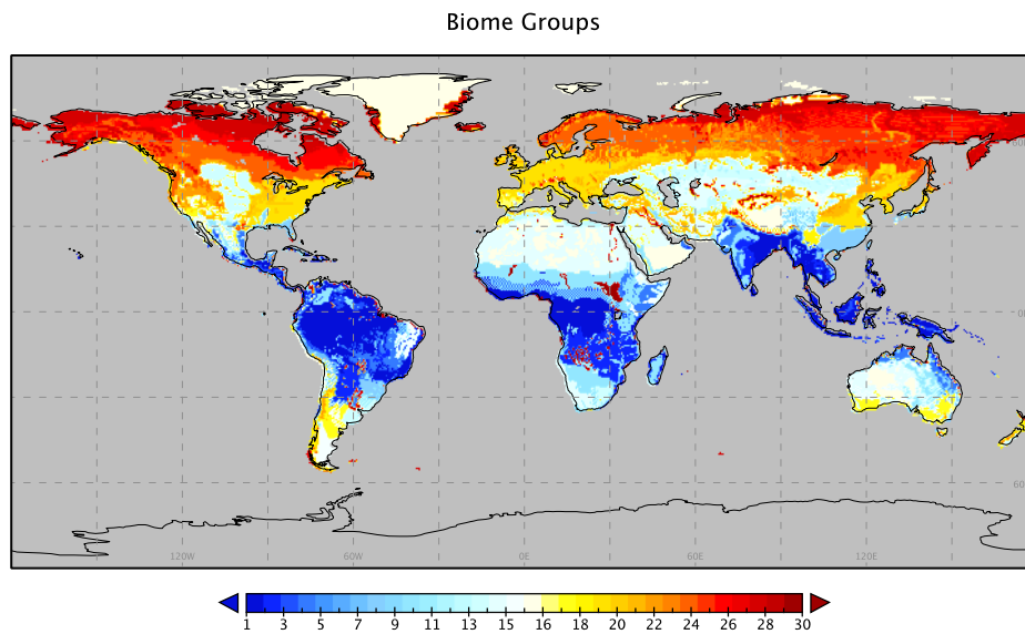
Figure 6. Distribution of the 31 biome groups on 0.5^\circ at global scale
