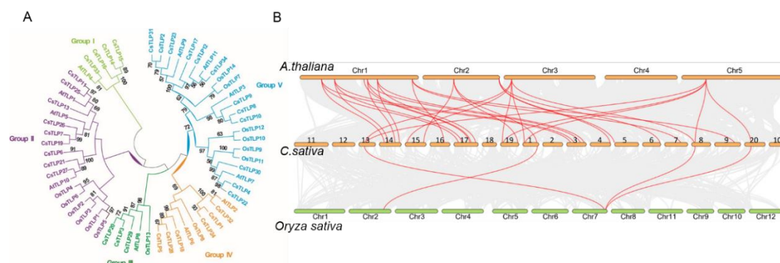
Figure 1. Phylogenetics and syntenic analysis of TLPs among C. sativa , A. thaliana and O. sativa
