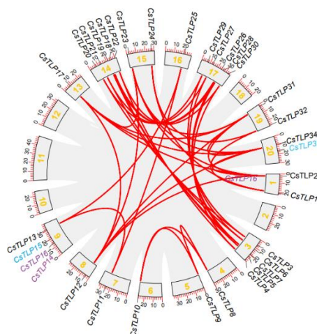
Figure 3. Chromosomal location and duplicated genes among 34 CsTLPs genes
