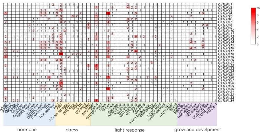
Figure 4. Cis-elements in putative promoter regions of TLPs gene in C. sativa
