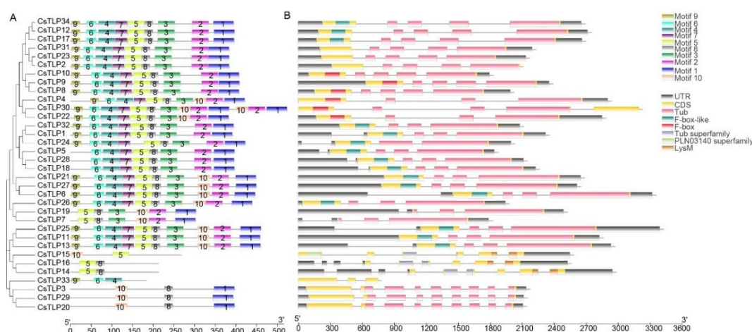
Figure 2. Phylogenetic tree, conserved protein motifs analysis, and gene structure of TLPs in C. sativa . A. The Neighbor joining method was utilized to construct the phylogenetic tree of C. sativa , with bootstrap values set to 1000. The Conserved protein motifs of CsTLP were also incorporated, with each motif being represented by a distinct color. B. Exon-intron structure and functional domains of the TLPs gene (yellow boxes represent exons, black lines represent introns, and specific colors represent different functional domains)
