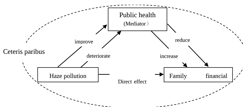
Figure 1. Theoretical model
