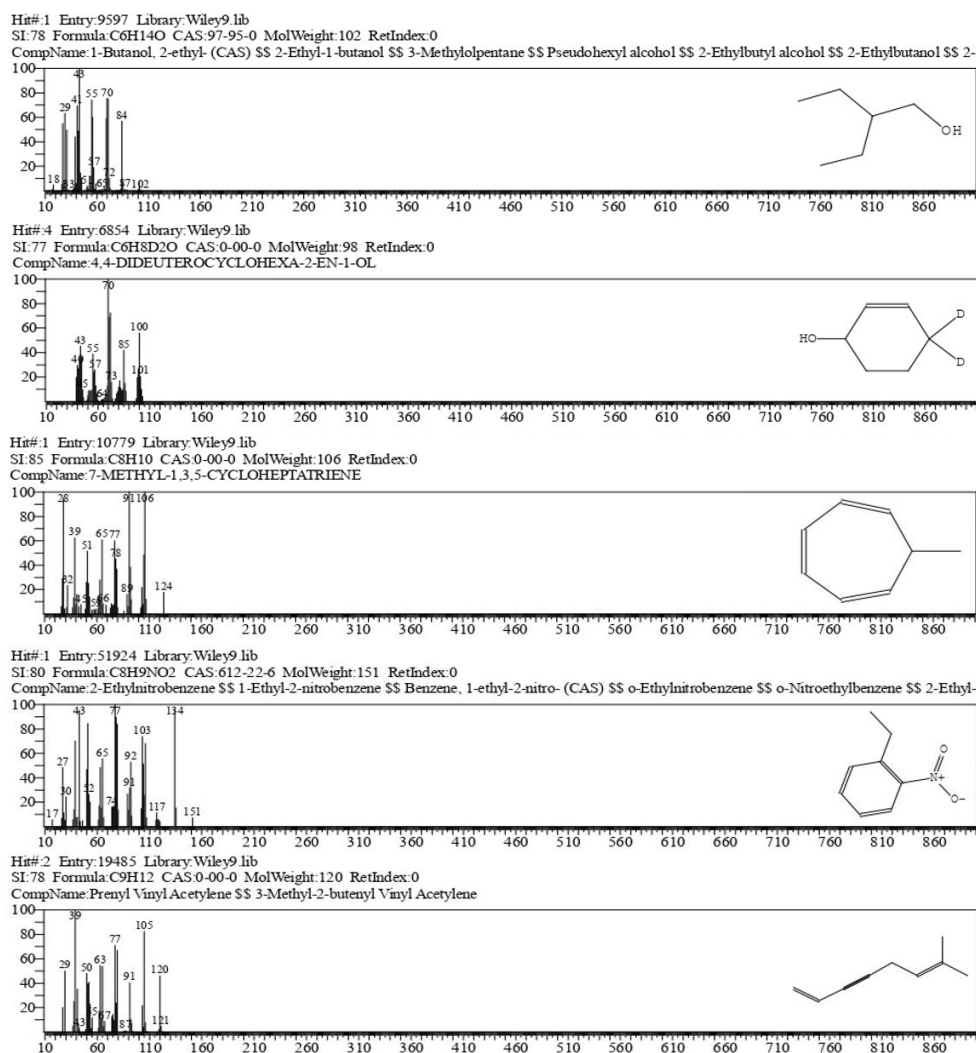
Figure 5. Shows the MS fragmentation form of Coffea arabica green bean compounds with high intensity and their molecular structures
