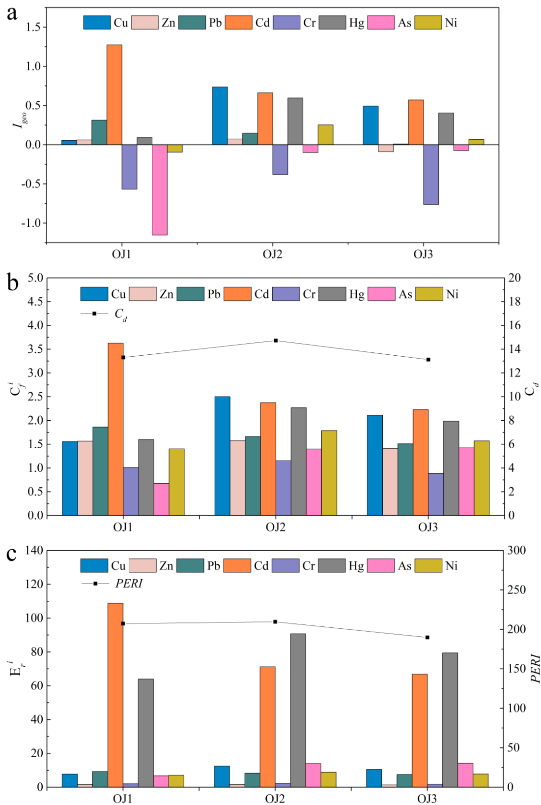
Figure 2. Geoaccumulation index (a), degree of contamination (b) and potential ecological risk index (c) of 8 heavy metals in surface sediments of Oujiang Estuary
