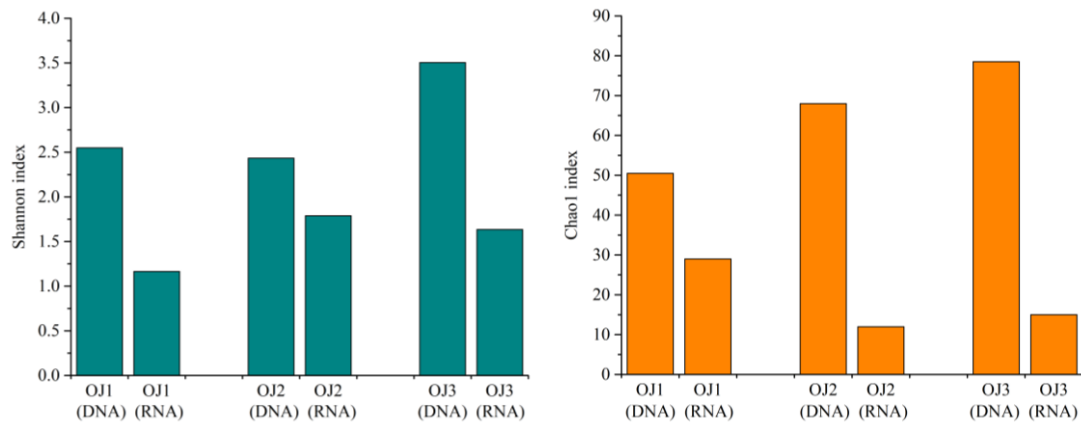
Figure 3. OTU-level Shannon index (a) and Chao1 index (b) of total and active foraminiferal community
