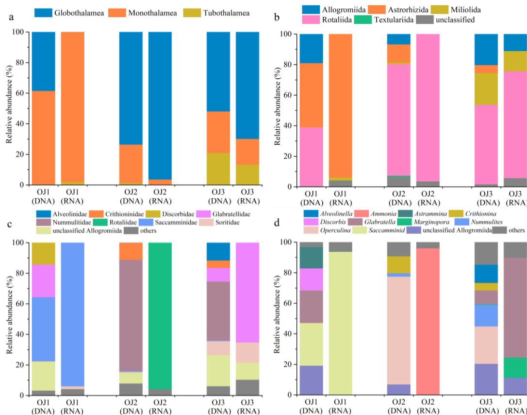
Figure 4. Total and active foraminiferal community composition in the sediment samples at the class (a), order (b), family (c) and genus (d) levels
