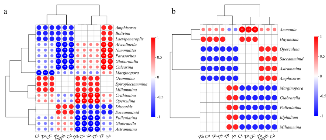
Figure 5. Heatmaps indicating the correlations between total (a) and active (b) benthic foraminifera at the genus level and environmental parameters. ** indicates p \leq 0.01
