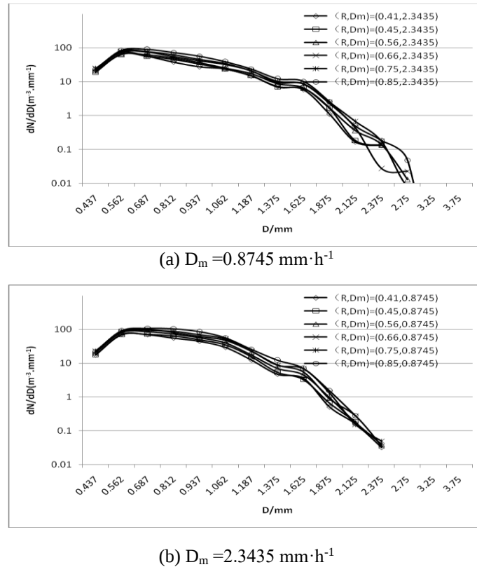
Figure 4. Multiple groups with the same median diameter D_m and different rainfall rate R
