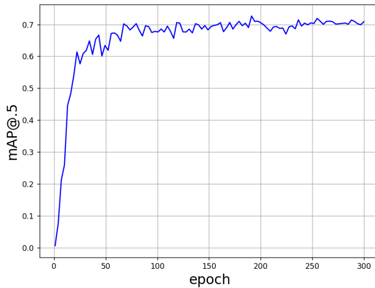
Figure 8. Improved mAP@0.5 -epoch curve
