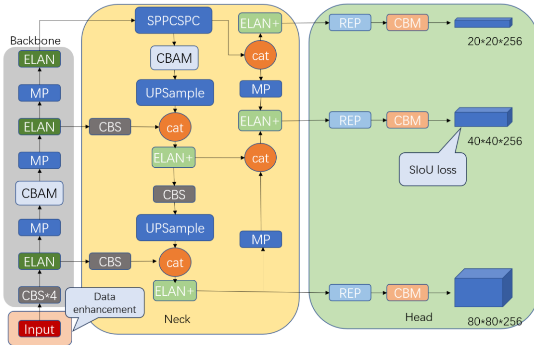
Figure 4. The improved YOLOv7 network structure
