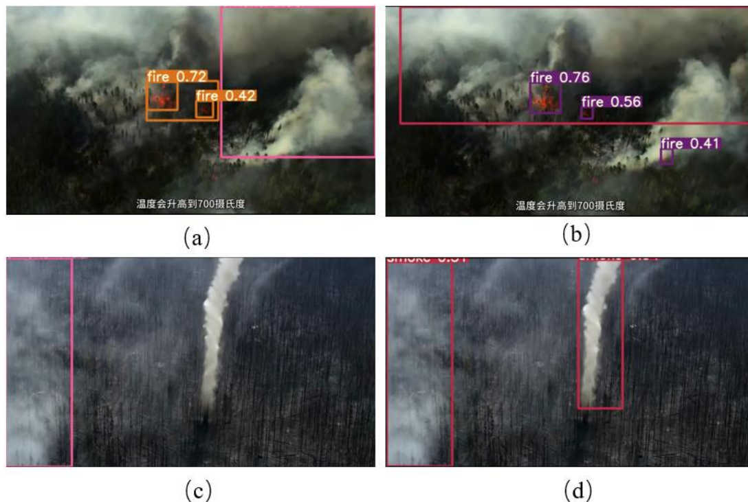
Figure 6. Comparison of detection performance before and after model improvement
