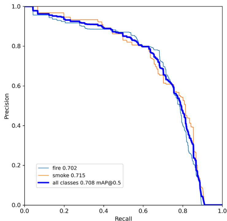
Figure 7. Improved P-R curve.
