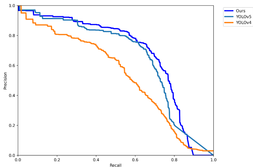
Figure 9. P-R curves of comparative experiments
