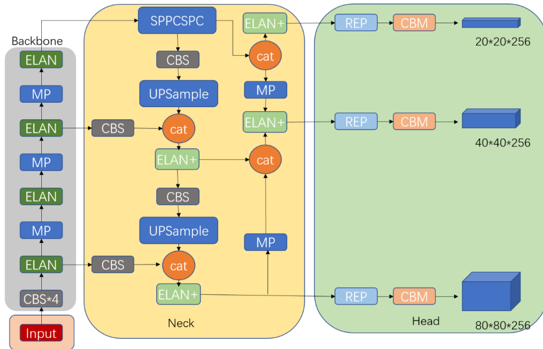
Figure 1. YOLOv7 network structure
