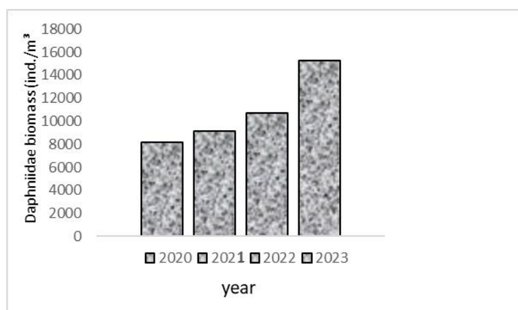
Figure 3. Annual changes of Daphniidae biomass (ind./m³)
