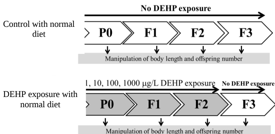
Figure 1. Experimental design of DEHP exposure for the multigenerational test of reproduction and growth in water flea ( M. macrocopa ). Maternal water fleas (P0) were exposed to different concentrations of DEHP, which were 1, 10, 100, and 1000 µg/L DEHP, respectively. Subsequently, the P0 water fleas at day 1 adulthood were transferred to the same concentration of DEHP-contained medium with normal diets for 8 days so that P0 could not produce offspring. Then, allowed P0's offspring (or F1) to reach adulthood for 1 day and then counted offspring number. Moreover, the offspring of P0 (F1) were treated with the same concentration of DEHP with the maternal exposed condition. For the next generation, F1 water fleas were placed in the same DEHP contained medium with normal diets and the procedures were performed as described in P0. Three water flea generations were exposed to DEHP; i.e. P0, F1, and F2. However, F3 progeny were transferred into the normal medium without DEHP
