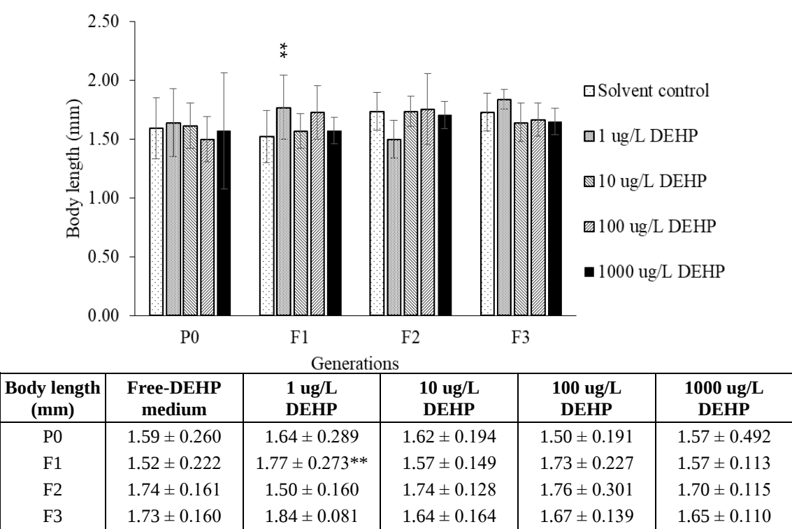
Figure 3. Body length of P0, F1, F2 M. macrocopa exposed to 1, 10, 100, and 1000 µg/L DEHP with normal diets. In addition, F3 M. macrocopa was transferred into a free-DEHP medium with normal diets. Three independent biological replicates were performed with at least three M. macrocopa per group. M. macrocopa was observed by capturing the images under an optical microscope with a 5x objective lens and eyepiece camera. The captured image was then analyzed by image software ToupView 3.7 for body length. Error bars indicate standard deviations. ANOVA and post hoc tests (Tukey HSD, LSD) were used for significant difference tests from solvent control (** indicate p < 0.01 )
