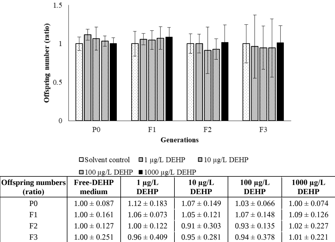
Figure 2. Offspring numbers (ratio) of neonates of P0, F1, and F2 M. macrocopa exposed to 1, 10, 100, and 1000 µg/L DEHP with normal diets. In addition, F3 M. macrocopa was transferred into a free-DEHP medium with normal diets. The ratio was calculated from the offspring number of each DEHP treatment divided by the offspring number of solvent control. Also, the ratio was calculated within the same generation. Error bars are standard deviations. ANOVA and post hoc test were used to obtain the significant difference from solvent control (0.1% v/v DMSO). The outcome of the post hoc test (Tukey HSD, LSD) was not displayed on the plots because there is no significant difference
